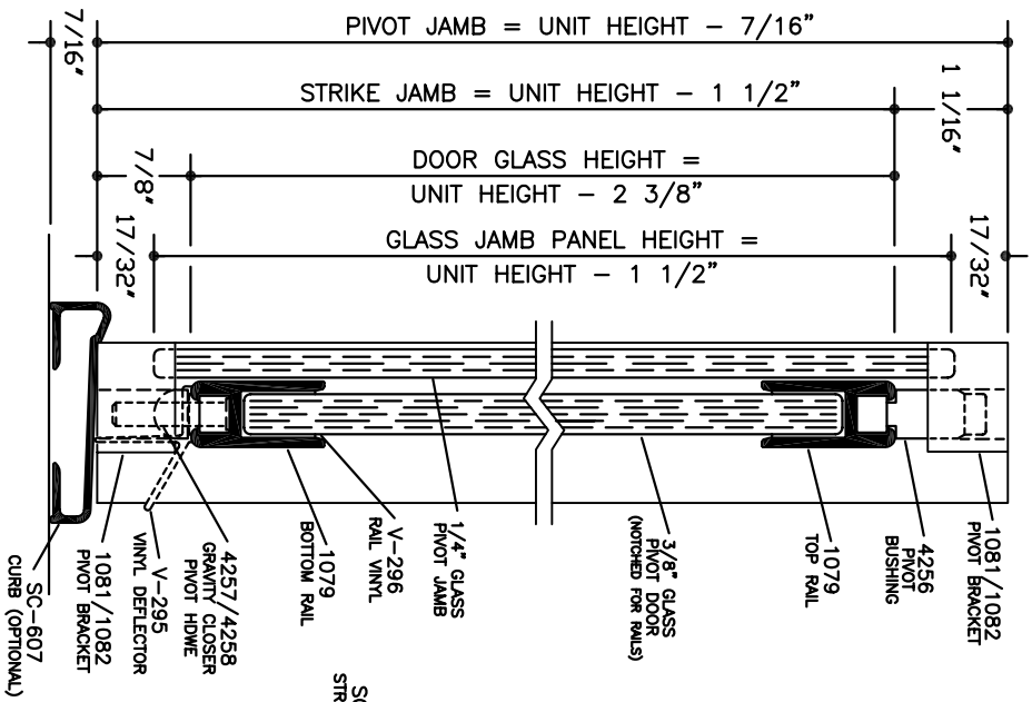
VERTICAL CROSS SECTIONS
