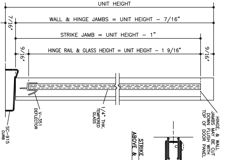
VERTICAL CROSS SECTIONS
