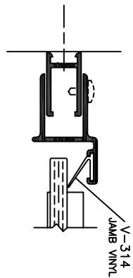
STRIKE JAMB DETAIL ABOVE & BELOW MAGNET
