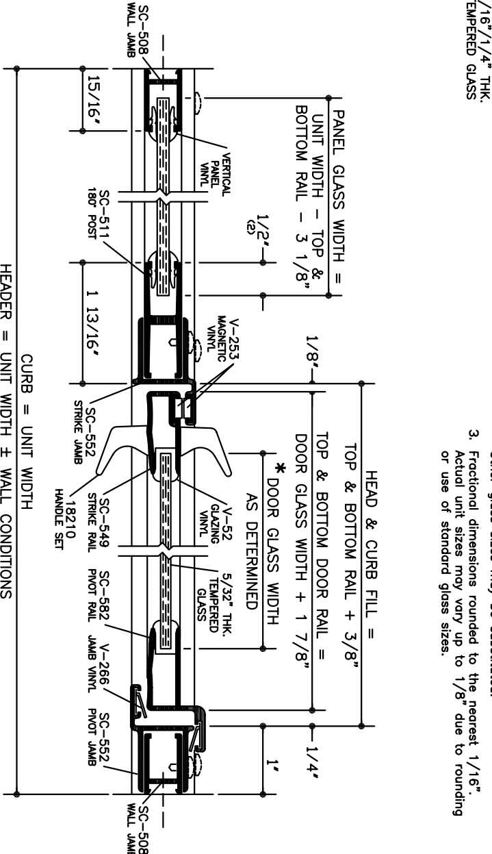
HORIZONTAL CROSS SECTION
