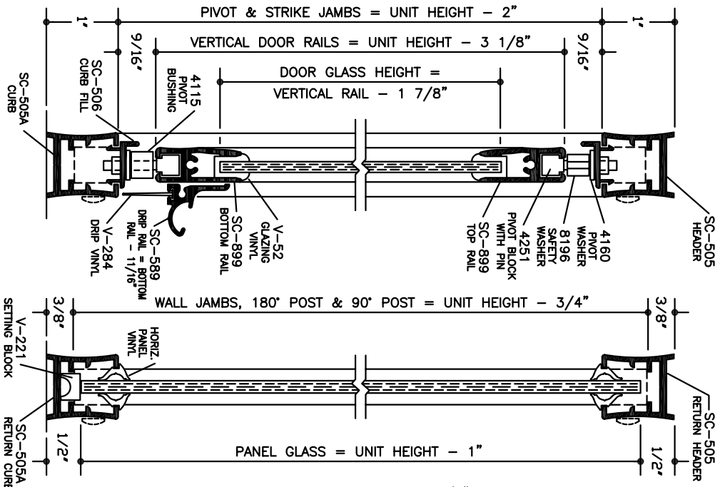
VERTICAL CROSS SECTION
